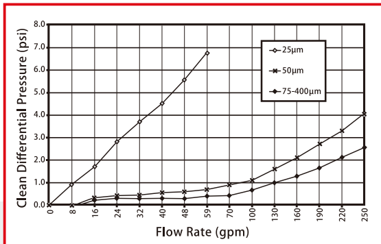
Pressure/Flow Curve
